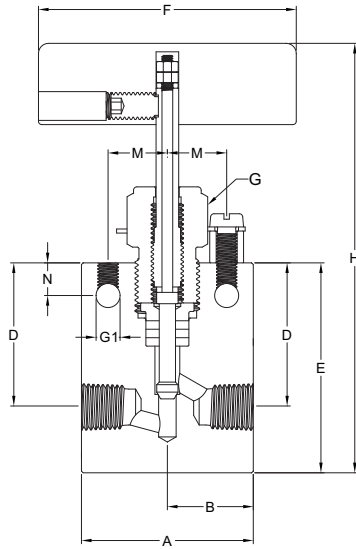
Dimensions (Straight)
