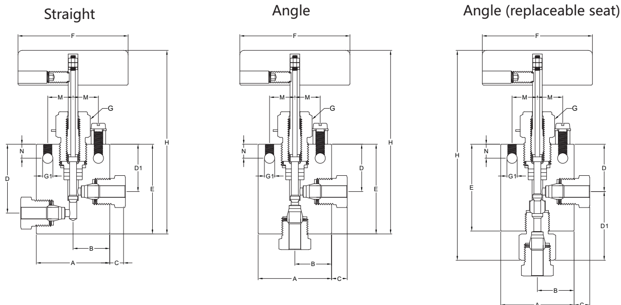
Dimensions (Straight)
