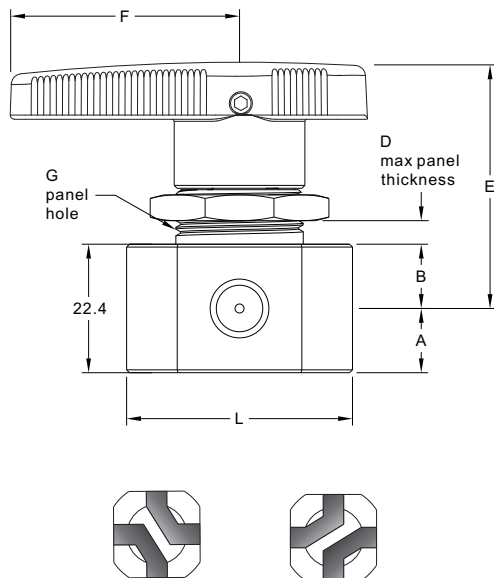
4-way Valve
