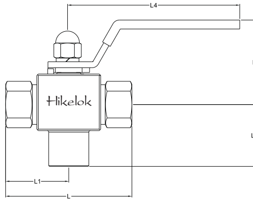
Vertical Pattern
