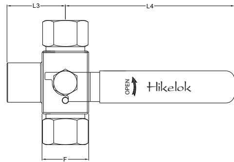
Horizontal Pattern
