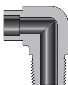
Male Elbows
