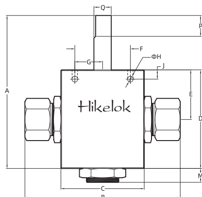
2-way Valves
