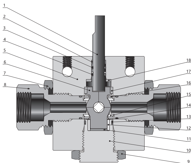
2-way Valves
