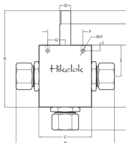
3-way Valves
