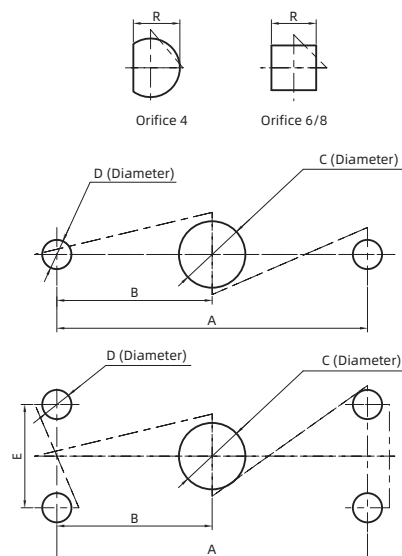
Ball stem connection
